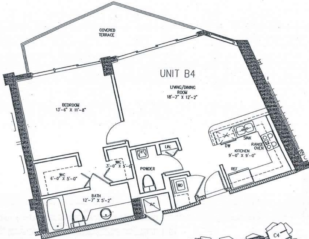
UNIT "B4" FLOOR PLAN
